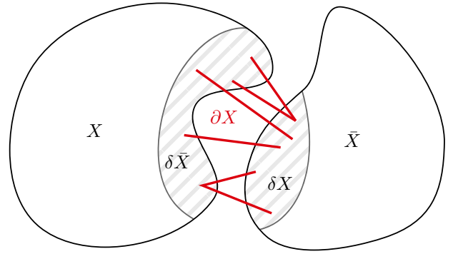
FIG. 2. A graph can be partitioned into two sets of vertices X and \bar{X} . The vertex boundary \delta X of X is the set of vertices outside of X that are directly connected to X , and similarly for \delta \bar{X} and \bar{X} . The edge boundary \partial X (red) of X (and \bar{X} ) is the set of edges that connect X to \bar{X} .
